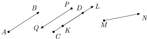
Рис. 17.2. \overline{AB} = \overline{CD} = \overline{KL} .
