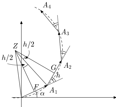
Рис. 22.3. \overline{OA_1} = \bar{a}_0 , \overline{A_1A_2} = \bar{a}_1, \dots, \overline{A_{10}A_{11}} = \bar{a}_{10} .
